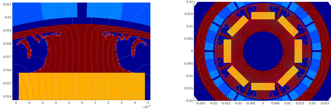
Figure 9: Final design after 375 iterations when applying algorithm [8], which uses the topological derivatives (67) and (93), to problem (4)–(5).
