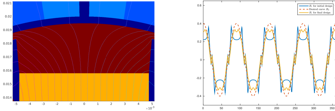
Figure 8: Left: Initial design. Right: Radial component of magnetic flux density in air gap for initial and final design and desired curve.
